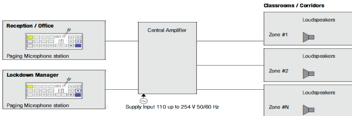
Diagram of School Lockdown Alarm System
